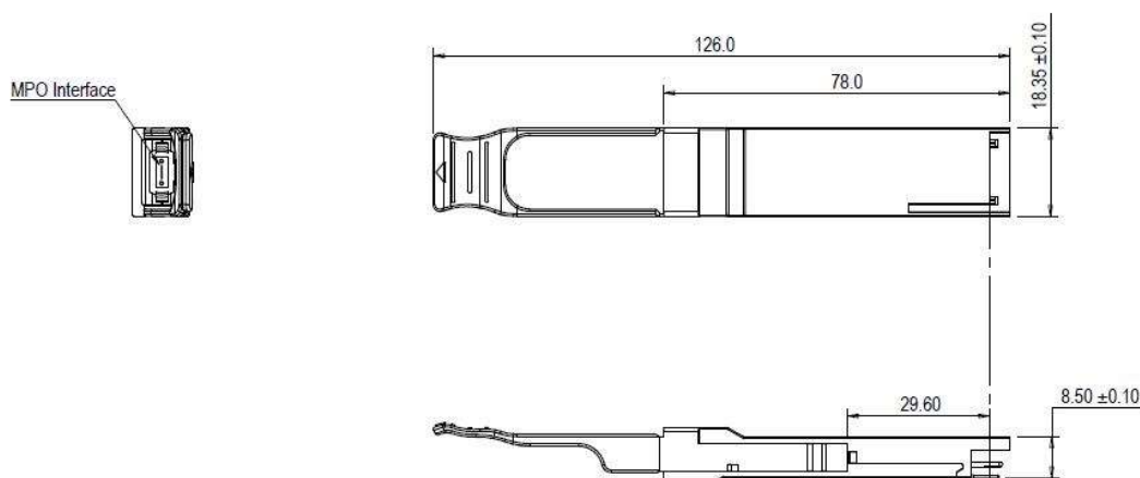
Figure 4. Mechanical Outline
