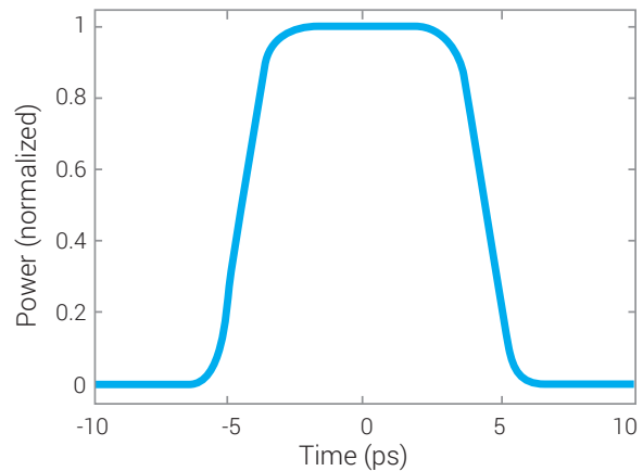
Examples of some of the pulse shapes which can be generated using a WaveShaper 1000A/SP in combination with a short pulse laser and appropriate compressive elements.
