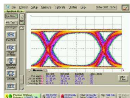
10 Gb/s Electrical Demodulated Eye Diagram
