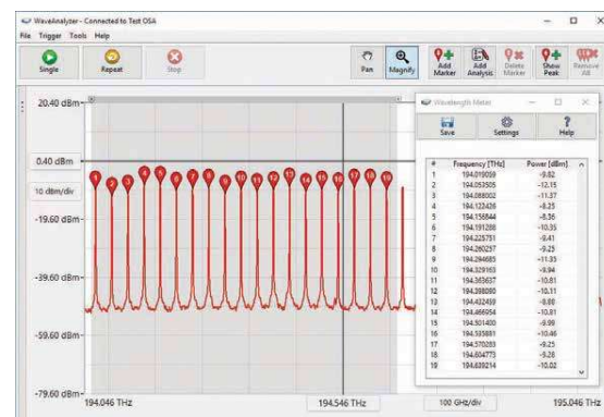
Wavelength Meter
