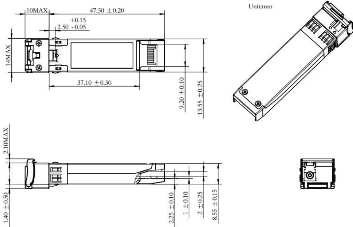
Figure 3 Package Outline
