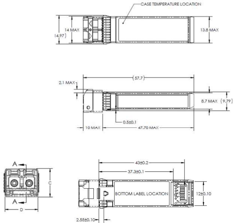
Figure 2. Mechanical Dimensions
