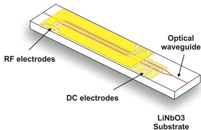
Schematic view of a LiNbO 3 intensity modulator chip
