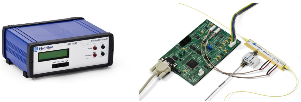
Left : MBC-DG-BT bench top bias controller Right : MBC-DG-board OEM bias control board
